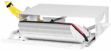
FIST-GSS3 Fiber Splice Panel, 3RU, 19 in, gray
