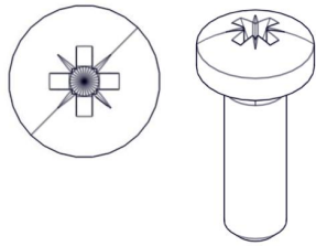
M5 x 16 (PZ-2)
